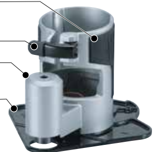
Replaceable, non-marring plastic base plate for protection of trimmer base and smooth sliding on work surface
